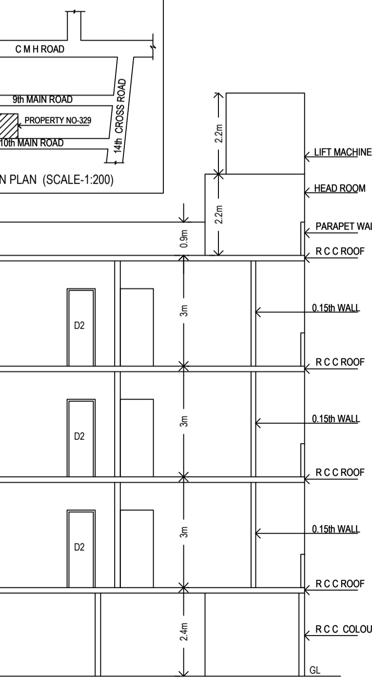
SECTION @ X-X
