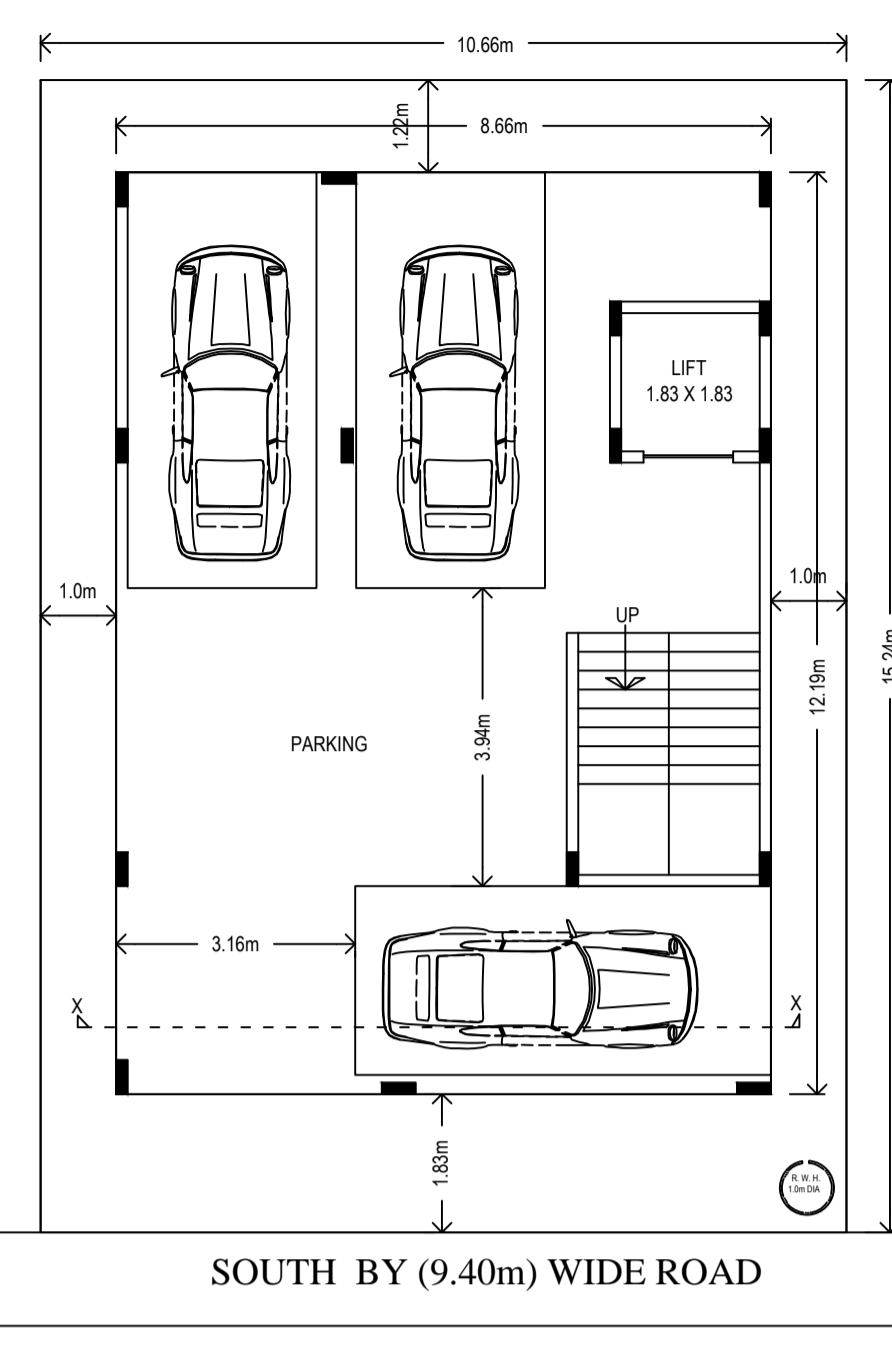
SOUTH BY (9.40m) WIDE ROAD
